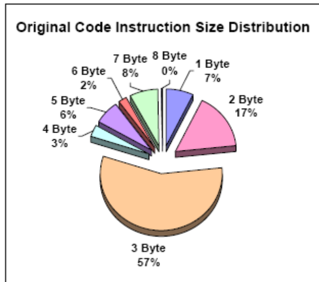
Figure 4.25: Overall Distribution of Instruction Sizes In the Original Five Benchmark Programs.
