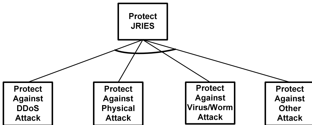
Figure 4.4: JRIES Protection Tree (High Level).
